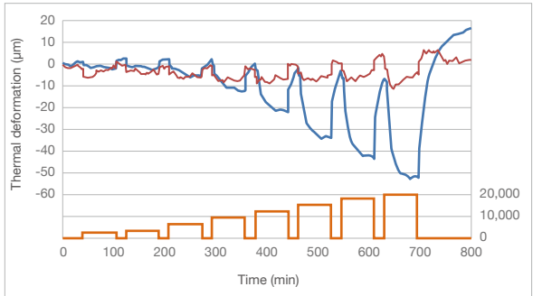
Z-axis thermal expansion chart
